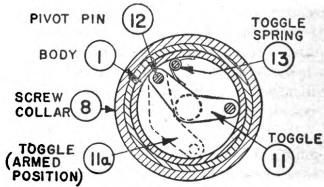
FIGURE 14.1.—PX32 push igniter.
